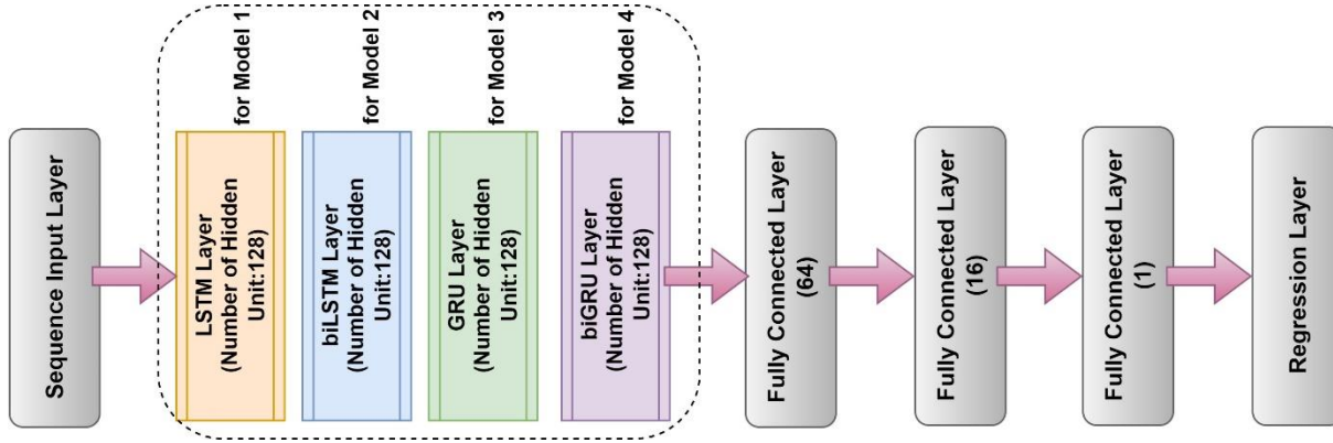
Figure 3. Deep network structure used in forecasting study.
